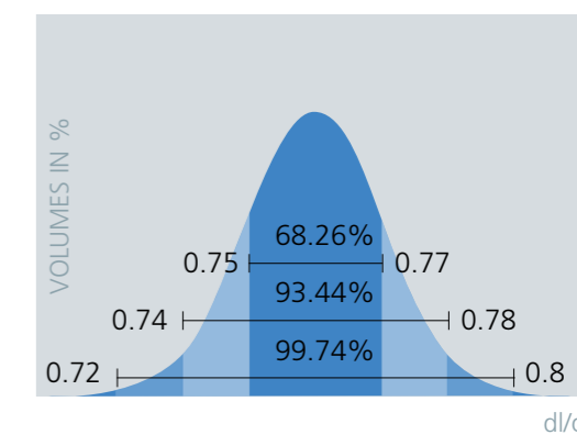
INPUT IV – TYPICAL DISTRIBUTION
