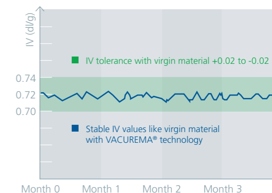
OUTPUT IV - WITH VACUREMA®
